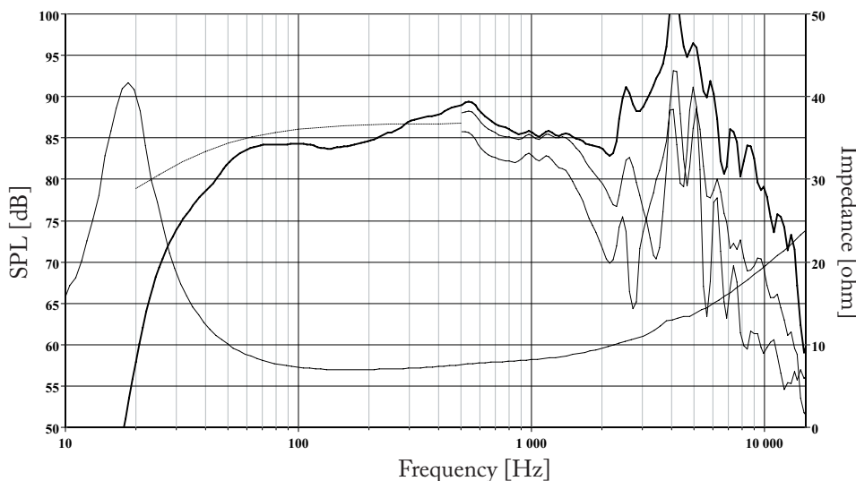
The frequency responses above show measured free field sound pressure in 0, 30, and 60 degrees angle using a 7L closed box. Input 2.83 VRMS, microphone distance 0.5m, normalized to SPL 1m. The dotted line is a calculated response in infinite baffle based on the parameters given for this specific driver. The impedance is measured in free air without baffle using a 2V sine signal.
